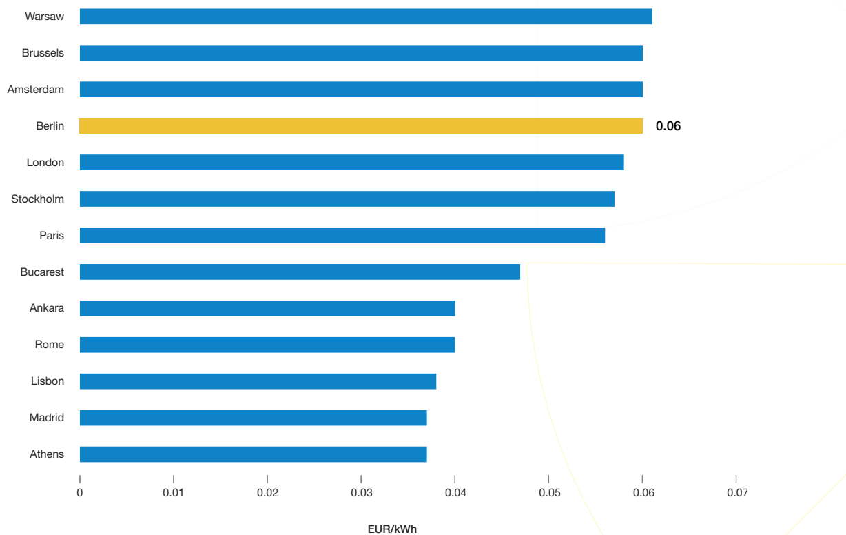
FIGURE 23 THEORETICAL LCOE IN DIFFERENT EUROPEAN COUNTRIES BASED ON GERMAN Q1/2017 TENDER RESULTS (EUR/kWh)
