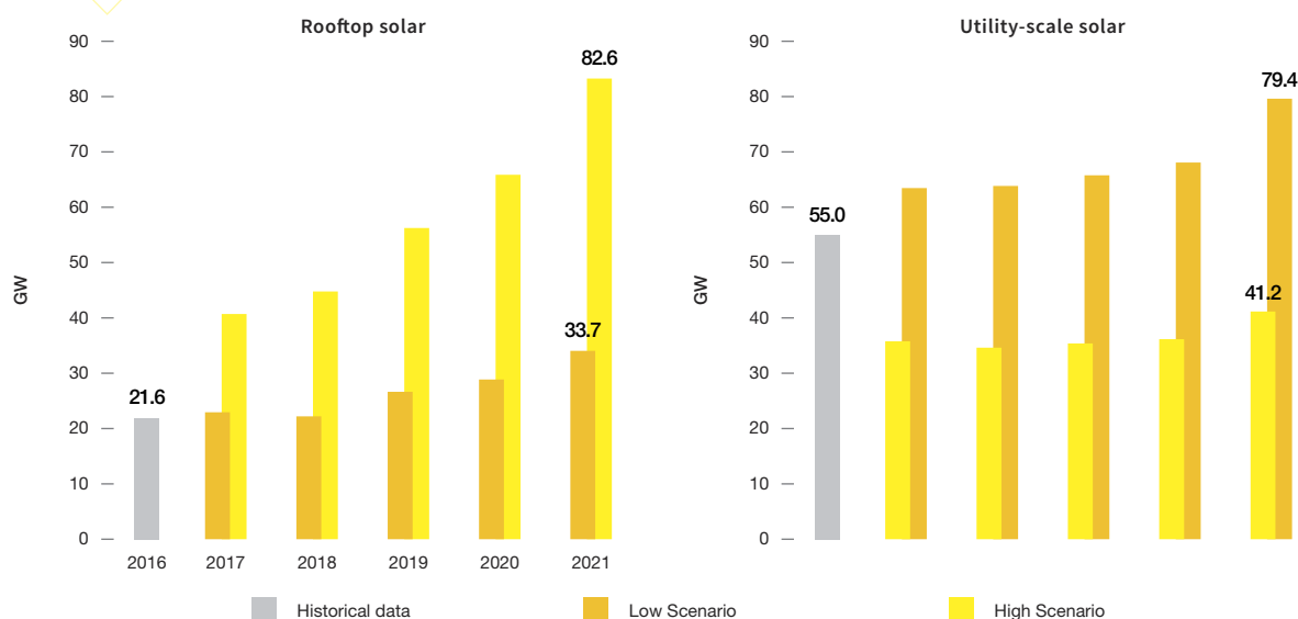
FIGURE 12 SCENARIOS FOR GLOBAL SOLAR PV ROOFTOP AND UTILITY SCALE SEGMENTS DEVELOPMENT 2016 - 2021
