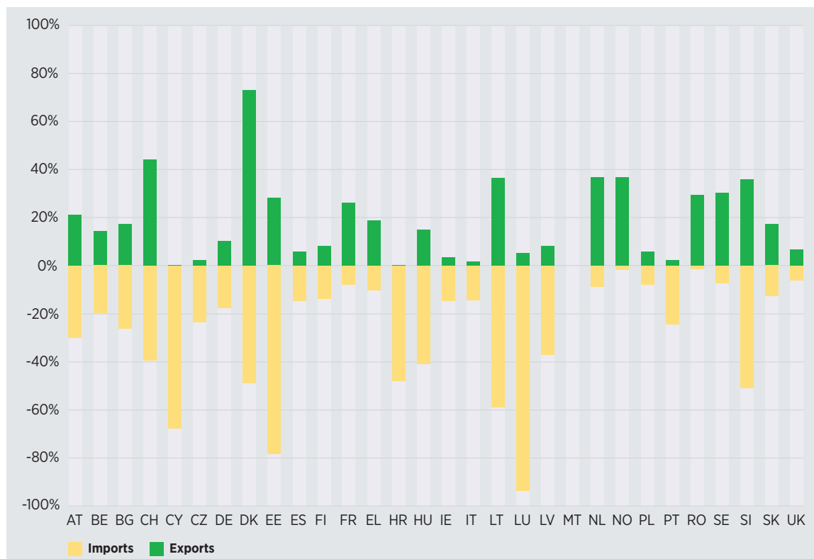
Figure 18: Power imports and exports by EU Member State in 2030 under REmap
