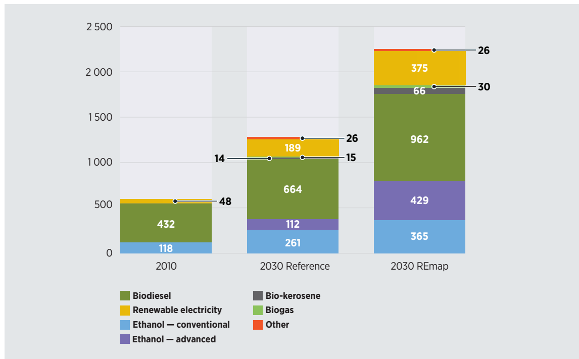
Figure 27: Final renewable energy consumption by source in the EU-28 transport sector in 2010 and in 2030 under the Reference Case versus REmap (PJ)
