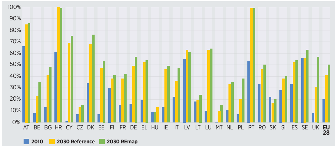
Figure 15: Renewable energy share in electricity generation by EU Member State in 2010 and in 2030 under the Reference Case versus REmap
