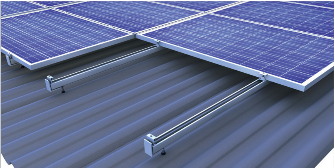
novotegra top-fix – single-rail clamping system with modules installed in landscape
