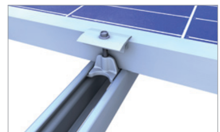
Middle clamp on C-rail
