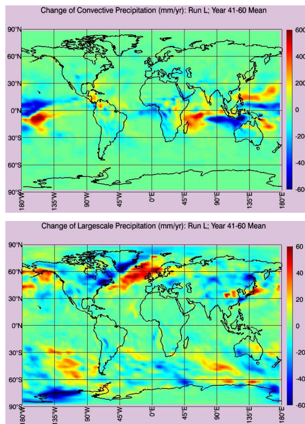
Fig. 9. Precipitation changes (Run L minus Run REF) for: convective precipitation (upper panel), and large-scale precipitation (lower panel). Both are in mm/yr and averaged over years 41–60.
