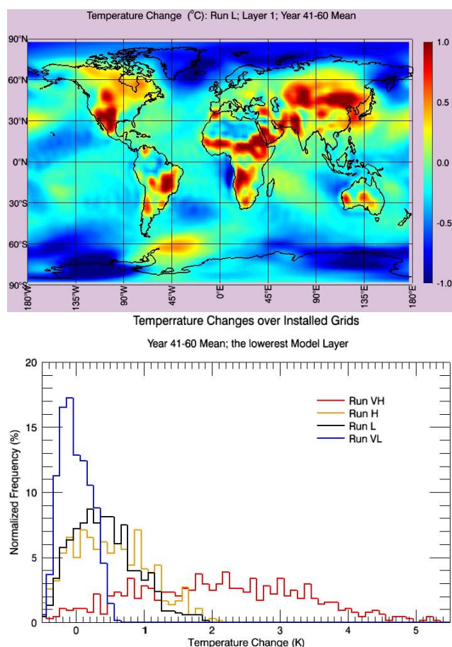
Fig. 2. Temperature changes (Run L minus reference, REF) in the lowest model layer resulting from large-scale deployment of wind turbines over land sufficient to generate 158 EJ/year of electric power (upper panel); and normalized frequency of temperature changes over the installation regions in Runs VH, H, L, and VL (lower panel). Both refer to averages over years 41–60.
