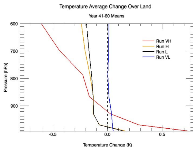
Fig. 3. Horizontally averaged temperature changes (relative to the reference, REF) over land in the 4 wind turbine installation runs. All data are 20-year means from year 41 to 60.
