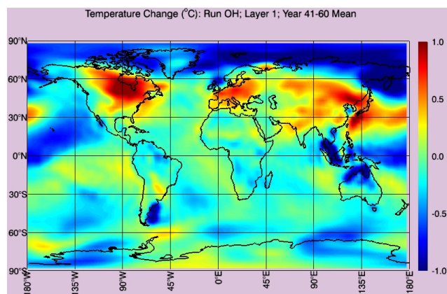
Fig. 8. Same as Fig. 2 (upper panel) but for Run OH.
