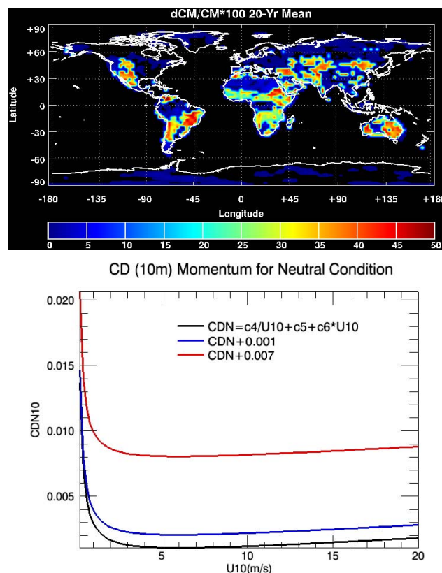
Fig. 7. Percentage changes of surface momentum drag coefficient ( d\text{CM}/\text{CM} \times 100 ) due to the simulated wind turbines over the land (upper panel); and surface momentum coefficients ( \text{CDN}_{10} ) without (black line) and with (Run OL, blue line; Run OH, red line) the simulated wind turbines over the ocean (lower panel).
