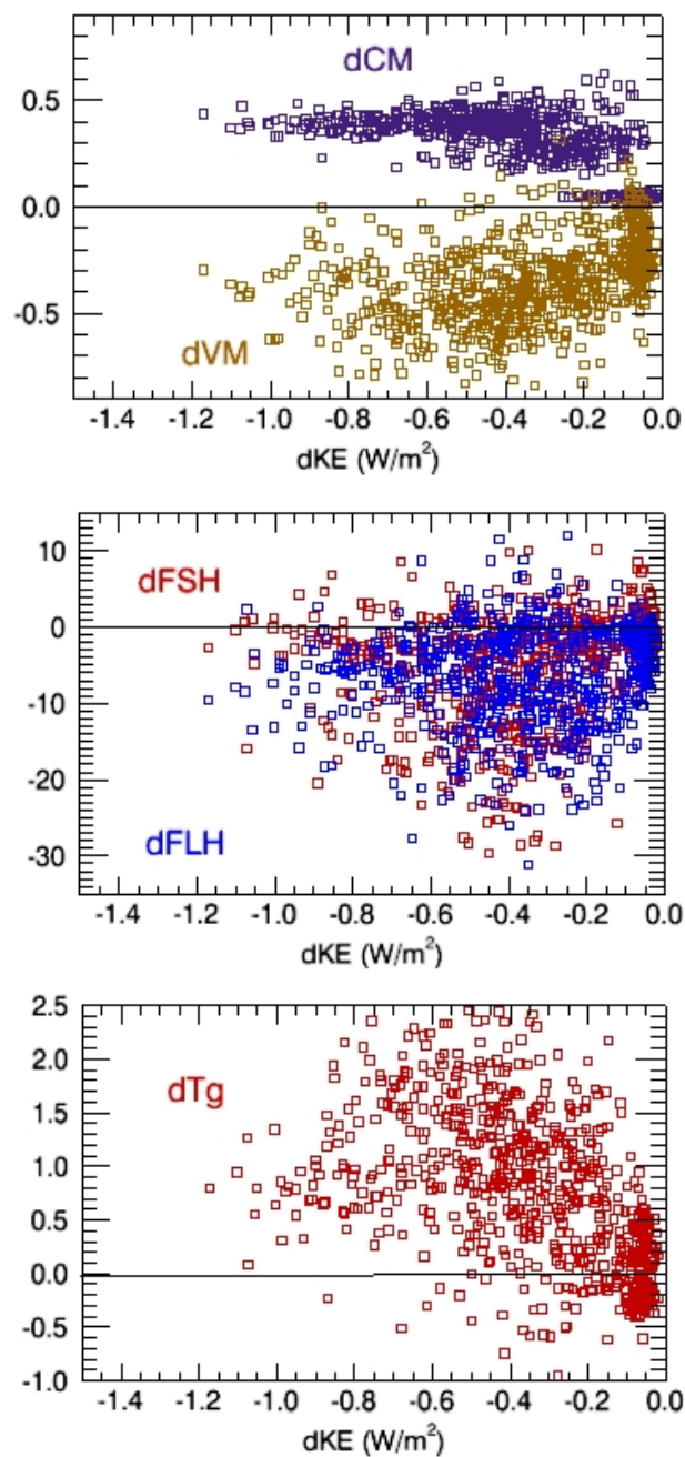
Fig. 5. Changes in surface momentum drag coefficient ( dCM ; unitless), wind magnitude ( dVM ; m/s), sensible ( dFSH ; W/m^2 ) and latent ( dFLH ; W/m^2 ) heat fluxes, and surface air temperature ( dTg ; K) over the model grids where the kinetic energy losses ( dKE ; W/m^2 ) due to wind turbines occur. Results shown are year 41–60 means of Run L minus Run REF.
