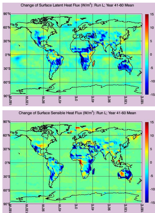
Fig. 6. Surface heat flux changes for Run L (Run L minus Run REF) for latent heat (upper panel) and sensible heat (lower panel) fluxes. Both panels are in \text{W/m}^2 and averaged over years 41–60.
