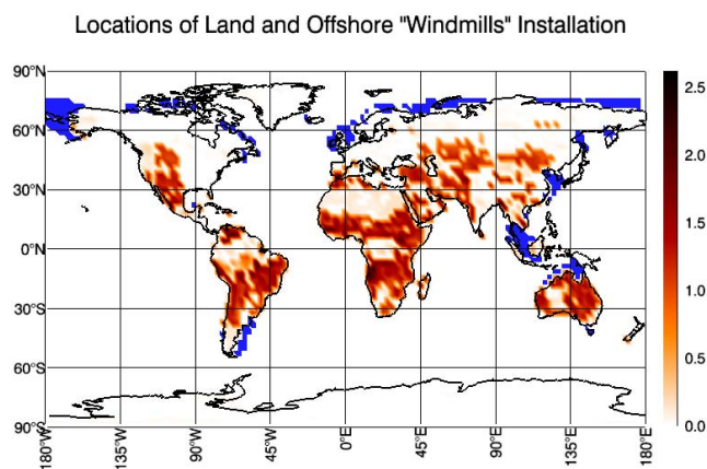
Fig. 1. Locations of land installations are indicated by the modeled change of surface drag coefficient (non-dimensional) averaged over the final 20 years of the 60-year Run L (see color code on right hand side). The drag values have been scaled by a factor of 1000. Also shown are the locations of offshore installation regions where the ocean depth is shallower than 200 m (blue shading).
