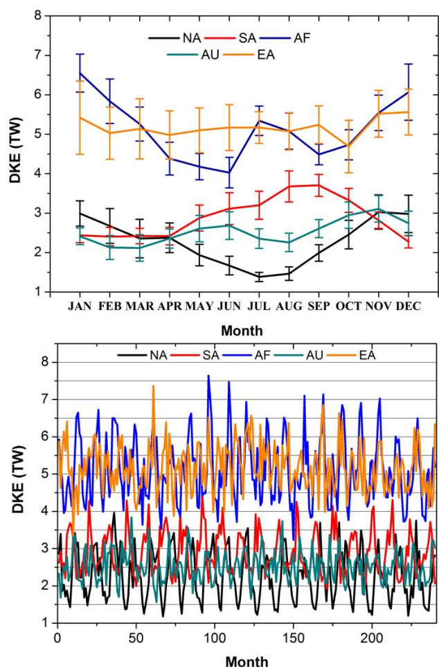
Fig. 10. Twenty-year (years 41–60) averages and standard deviations (upper panel), and all values (lower panel), of the monthly mean wind power consumption ( DKE=dKE/dt , Eq. 1) by simulated wind turbines installed in various continents: North America (NA), South America (SA), Africa and Middle East (AF), Australia (AU), and Eurasia (EA).
