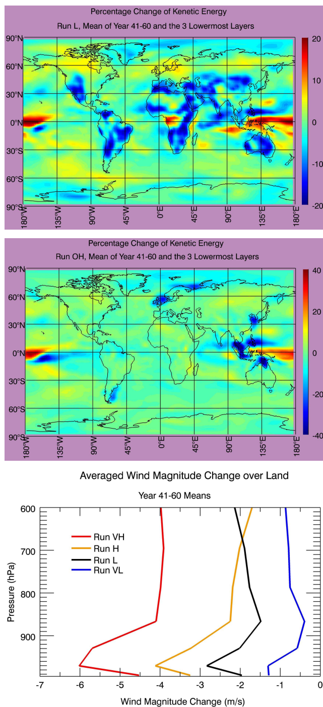
Fig. 4. The changes in the kinetic energy per unit mass are shown in the upper panel for Run L, and the middle panel for Run OH. Also shown in the lower panel are the horizontally averaged wind magnitude changes (derived from the kinetic energy per unit mass change) over land in the 4 wind turbine installation runs. All data are 20-year means from year 41 to 60.
