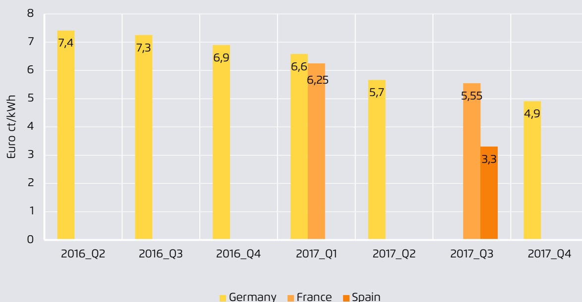
Solar PV auction results 2016-2017 (average prices, ground-mounted installations)
