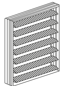
D2 - Frangisole orizzontale a cellule. Angoli prestabiliti e variabili. Collegabile alle facciate continue METRA Building ed alla muratura. D2 - Horizontal unit sunblades. Angles are present and variable. Can be connected to the METRA Building curtain walls and to the wall.
