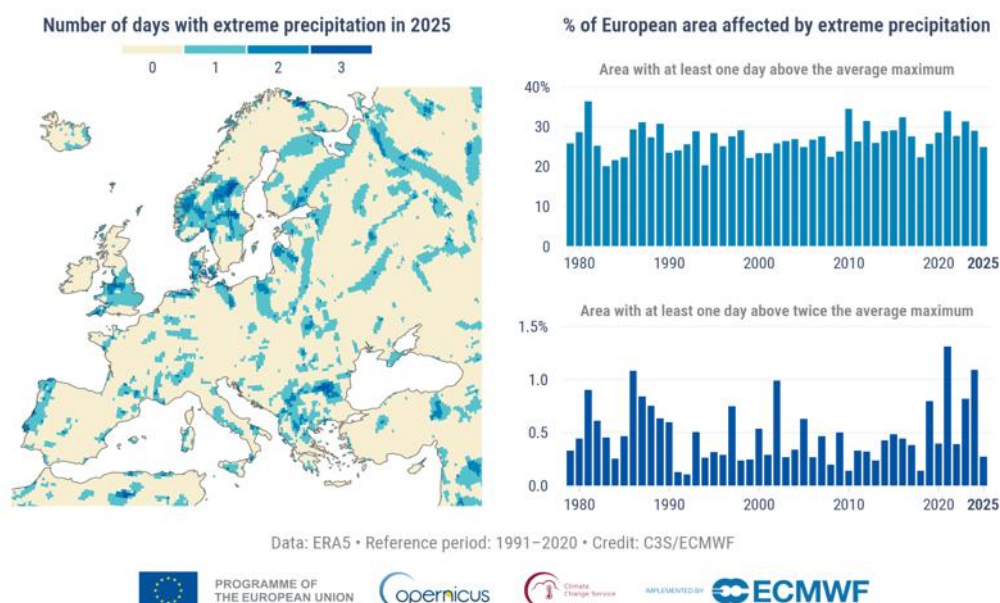
Figure 9.3. (Left) Map showing the total number of days with extreme precipitation across Europe in 2025. ‘Extreme precipitation’ refers to a day with total precipitation exceeding the average annual maximum daily precipitation during the 1991–2020 reference period. (Right) Annual time series showing the percentage of Europe’s land area (shown in the map) that experienced at least one day of extreme precipitation each year from 1979 to 2025. The time series show the area affected by daily precipitation exceeding one (top) and two (bottom) times the average annual maximum. Data: ERA5. Credit: C3S/ECMWF.
