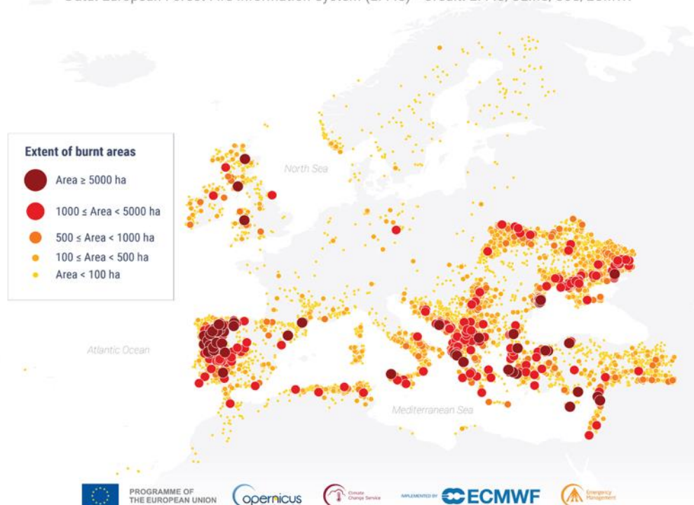
Figure 6.2. Distribution and extent of burnt areas across Europe and the Mediterranean 16 in 2025. Data: European Forest Fire Information System (EFFIS). Credit: EFFIS/CEMS/C3S/ECMWF.
