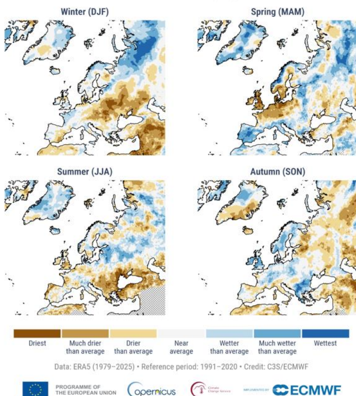
Figure 9.2a. Anomalies and extremes in seasonal precipitation in 2025. The extreme categories ('wettest' and 'driest') are based on rankings for 1979–2025. The other categories describe how precipitation compares to the distribution during the 1991–2020 reference period. 'Much wetter/drier than average' – wetter/drier than 90% of precipitation values; 'wetter/drier than average' – than 66% of precipitation values; 'near average' – within the middle 33%. Data: ERA5. Credit: C3S/ECMWF.
