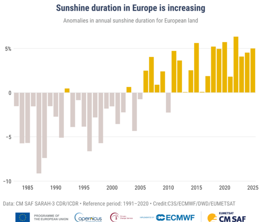
Figure 7.3. Annual sunshine duration anomalies (%) for Europe for 1983–2025, relative to the average for the 1991–2020 reference period. The anomalies are for land areas only and expressed as a percentage above or below average. Data: CM SAF SARA3-3 CDR/ICDR Credit: C3S/ECMWF/DWD/EUMETSAT.
