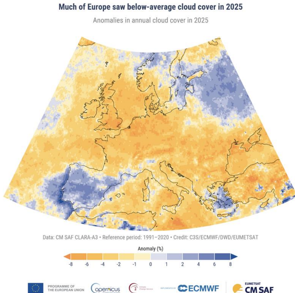
Figure 7.2. Average annual cloud cover fraction anomalies (%) over Europe for 2025, relative to the average for the 1991–2020 reference period. Data: CLARA-A3 CDR/ICDR. Credit: C3S/ECMWF/DWD/EUMETSAT.
