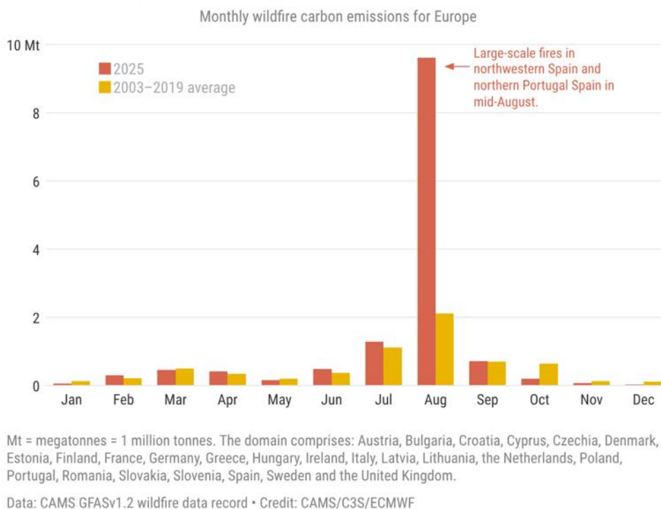
Figure 6.3. Estimated total monthly wildfire carbon emissions for Europe in 2025 (red) compared to the monthly average emission for the 2003–2019 reference period (yellow). Data: CAMS GFASv1.2 wildfire data record. Credit: CAMS/C3S/ECMWF.
