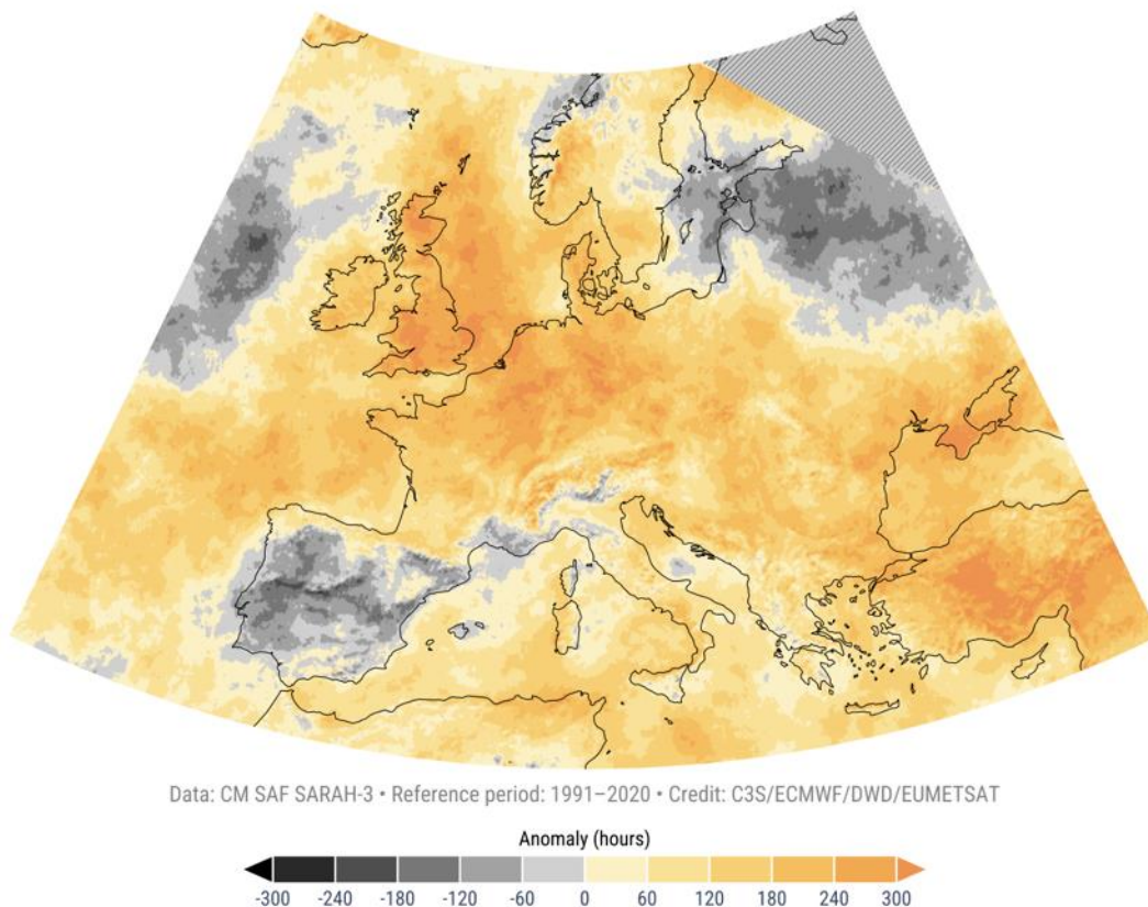
Figure 7.1. Sunshine duration anomalies (hours) over Europe for 2025, relative to the average for the 1991–2020 reference period. Grey hatching in the top right corner of the map indicates missing data. Data: CM SAF SARA3-3 CDR/ICDR. Credit: C3S/ECMWF/DWD/EUMETSAT.
