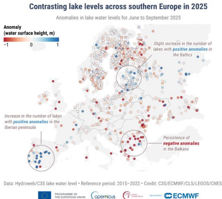
Figure 12.2. Lake water level (red and blue dots) anomalies (metres) in Europe for June–September, relative to the average for the 2015–2022 reference period. Data: Hydroweb, C3S lake water level. Credit: C3S/ECMWF/CLS/LEGOS/CNES.
