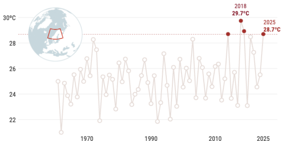
Average maximum temperature in July for sub-Arctic Fennoscandia, 1961–2025
