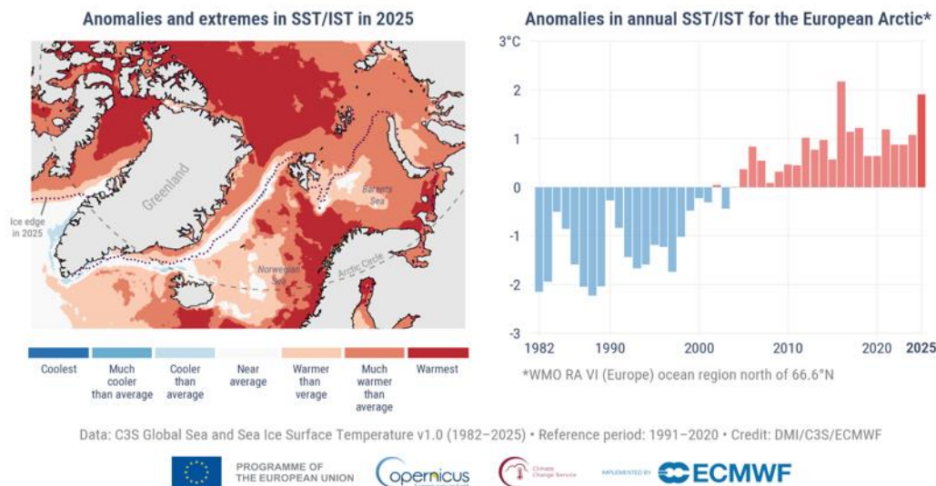
Figure 16.2. (Left) Anomalies and extremes in annual sea surface temperature (SST) and sea ice surface temperature (IST) in 2025. The extreme categories ('coolest' and 'warmest') are based on rankings for 1982–2025. The other categories describe how the temperatures compare to their distribution during the 1991–2020 reference period. 'Much cooler/warmer than average' – cooler/warmer than 90% of temperatures; 'cooler/warmer than average' – than 66% of temperatures; 'near average' – within the middle 33%. (Right) Annual SST/IST anomalies for the WMO RA VI (Europe) ocean region north of the Arctic Circle from 1982 to 2025, relative to the average for the 1991–2020 reference period. Data: C3S Global Sea and Sea Ice Surface Temperature v1.0. Credit: DMI/C3S/ECMWF.
