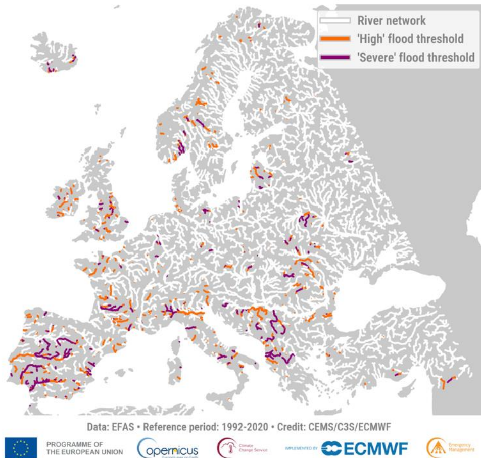
Figure 11.5. Rivers with upstream areas larger than 1000 km 2 (white), and those where the river flow exceeded the 'high' (five-year return period) (orange) and 'severe' (20-year return period) (purple) flood thresholds on any day across 2025. Data: EFAS. Credit: CEMS/C3S/ECMWF.
