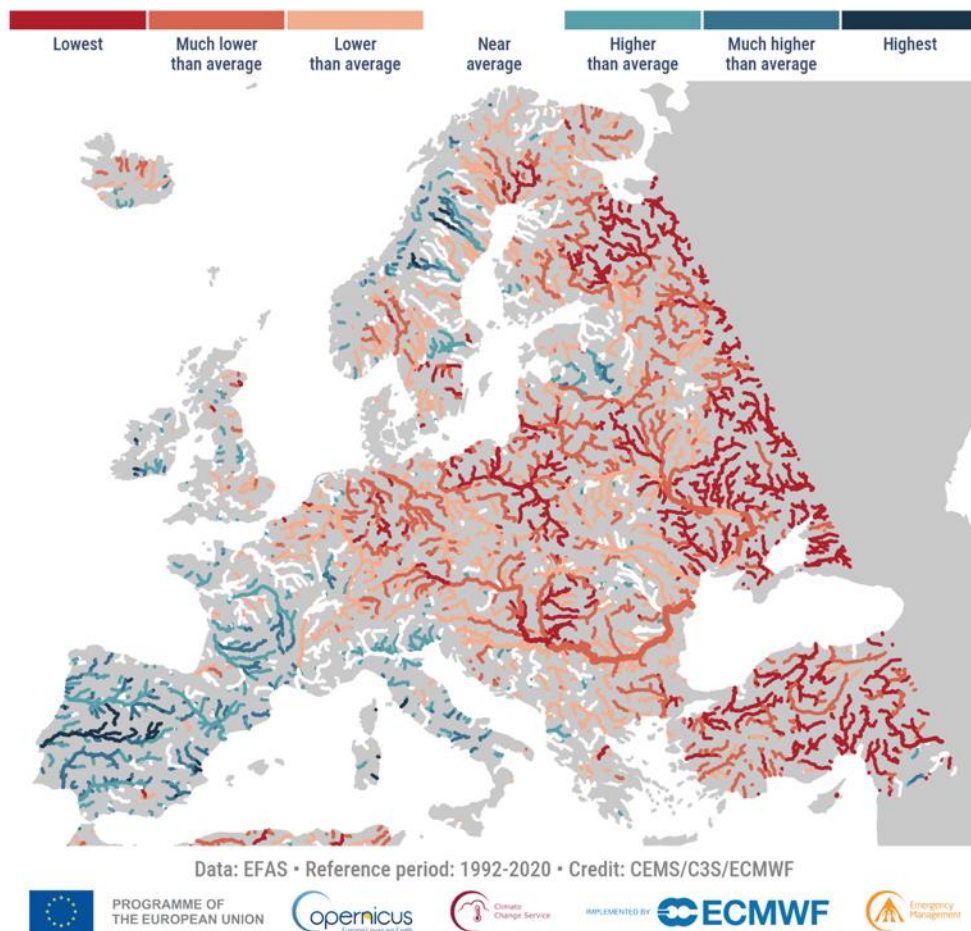
Figure 11.2. Anomalies and extremes in annual average river flow in 2025. The extreme categories ('highest' and 'lowest') are based on rankings for 1992–2025. The other categories describe how river flow compares to the distribution during the 1992–2020 reference period. 'Much higher/lower than average' – higher/lower than 90% of river flow values; 'higher/lower than average' – than 66% of river flow values; 'near average' – within the middle 33%. Only rivers with drainage areas greater than 1000 km 2 are shown. Data: EFAS. Credit: CEMS/C3S/ECMWF.
