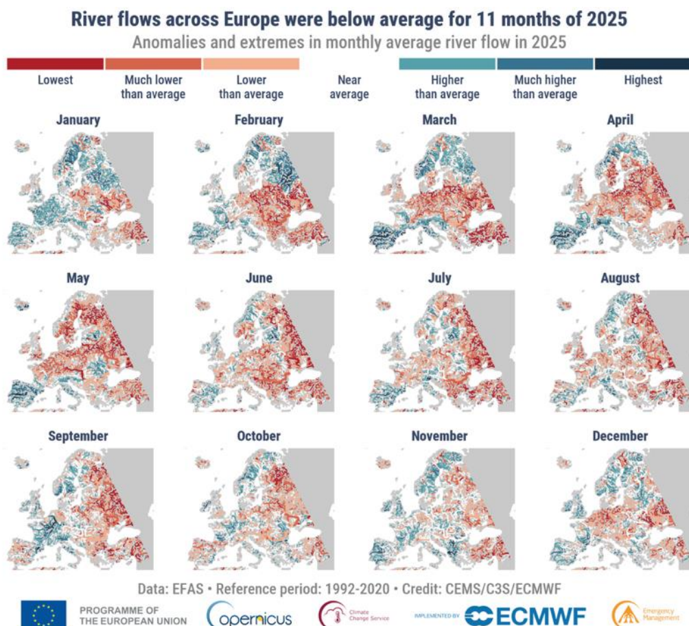
Figure 11.3. Anomalies and extremes in monthly average river flow in 2025. The extreme categories ('highest' and 'lowest') are based on rankings for 1992–2025. The other categories describe how river flow compares to the distribution during the 1992–2020 reference period. 'Much higher/lower than average' – higher/lower than 90% of river flow values; 'higher/lower than average' – than 66% of river flow values; 'near average' – within
