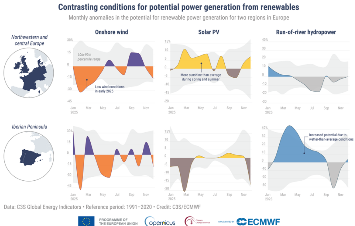
Figure 8.4. Monthly anomalies in the potential for power generation (capacity factor) from onshore wind, solar photovoltaic (PV) and run-of-river hydropower, averaged over (top) northwestern and central Europe (Ireland, the United Kingdom, France, Belgium, the Netherlands, Luxembourg, Germany and Denmark) and (bottom) the Iberian Peninsula (Spain and Portugal). The anomalies are expressed as percentages relative to the 1991–2020 reference period. Grey shading indicates the 10–90th percentile range of the 1991–2020 reference period, which represents the majority of historical values excluding the highest and lowest 10%. Data: C3S Global Energy Indicators. Credit: C3S/ECMWF.
