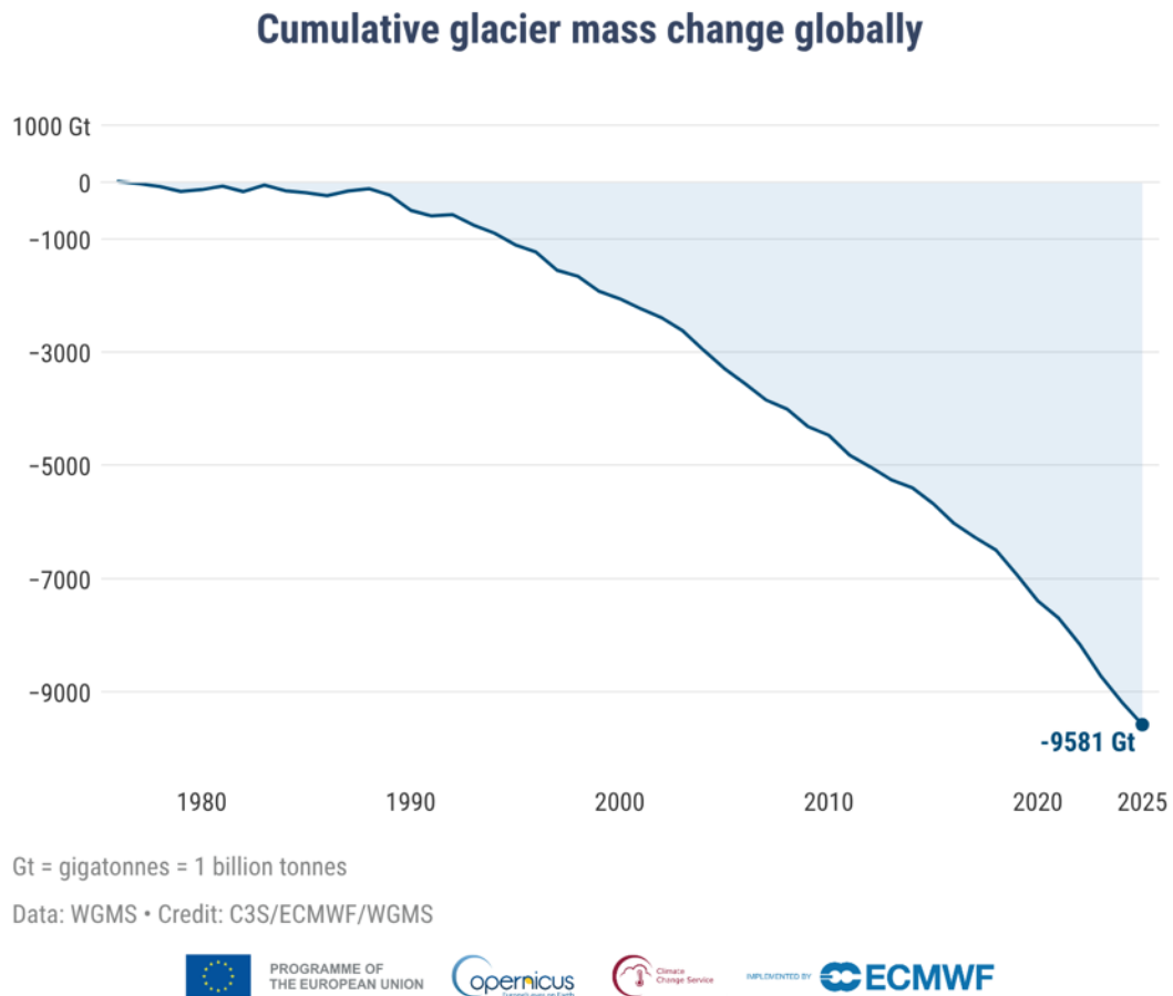
Figure 14.3. Cumulative global glacier mass changes from 1976 to 2025. Data: WGMS. Credit: WGMS/C3S/ECMWF.
