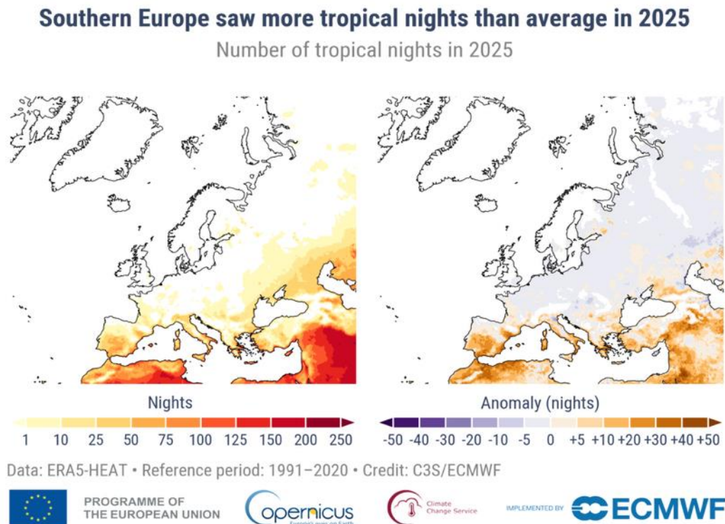
Figure 5.2. (Left) Number of tropical nights in 2025 and (right) associated anomalies relative to the average for the 1991–2020 reference period. Tropical nights are those during which the temperature does not fall below 20°C. Data: ERA5-HEAT. Credit: C3S/ECMWF.
