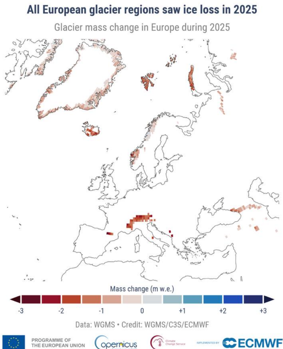
Figure 14.1. Glacier mass changes across Europe in the 2025 hydrological year. Positive (blue) and negative (red) mass change is shown in metre water equivalent (m w.e.; 1 m w.e. = 1000 kg per square metre) averaged over the glacier area within 0.5^\circ \times 0.5^\circ grid cells. For Greenland, the mass change estimates include the peripheral glaciers but not the Greenland Ice Sheet. In Europe, the hydrological year runs from 1 October to 30 September. Data: WGMS. Credit: WGMS/C3S/ECMWF.
