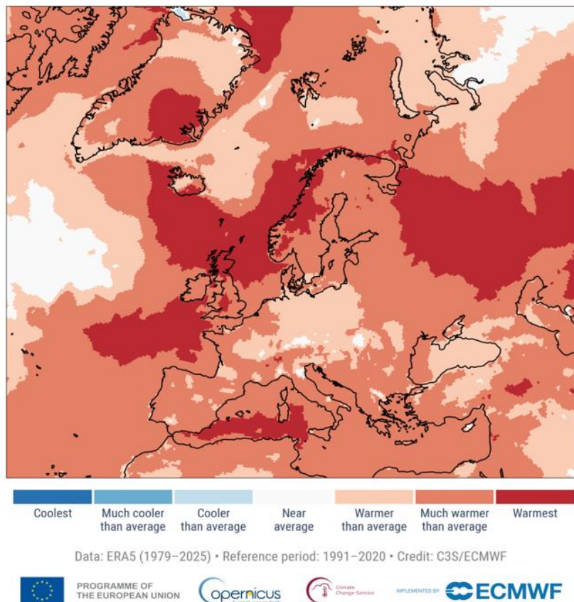
Figure 4.1a. Anomalies and extremes in annual surface air temperature in 2025. The extreme categories ('coolest' and 'warmest') are based on rankings for 1979–2025. The other categories describe how the temperatures compare to their distribution during the 1991–2020 reference period. 'Much cooler/warmer than average' – cooler/warmer than 90% of temperatures; 'cooler/warmer than average' – than 66% of temperatures; 'near average' – within the middle 33%. Data: ERA5. Credit: C3S/ECMWF.
