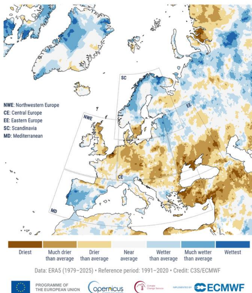
Figure 9.1a. Anomalies and extremes in annual precipitation in 2025. The extreme categories (‘wettest’ and ‘driest’) are based on rankings for 1979–2025. The other categories describe how precipitation compares to the distribution during the 1991–2020 reference period. ‘Much wetter/drier than average’ – wetter/drier than 90% of precipitation values; ‘wetter/drier than average’ – than 66% of precipitation values; ‘near average’ – within the middle 33%. The dashed boxes outline the five European subregions discussed in the text. Data: ERA5. Credit: C3S/ECMWF.
