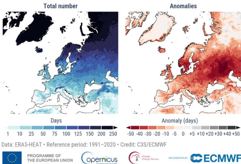
Figure 5.3. (Left) Number of days with at least 'strong' cold stress in 2025 and (right) associated anomalies relative to the average for the 1991–2020 reference period. A day with at least strong cold stress has a minimum feels-like temperature, based on the Universal Thermal Climate Index (UTCI) of -13^{\circ}\text{C} or lower. Data: ERA5-HEAT. Credit: C3S/ECMWF.
