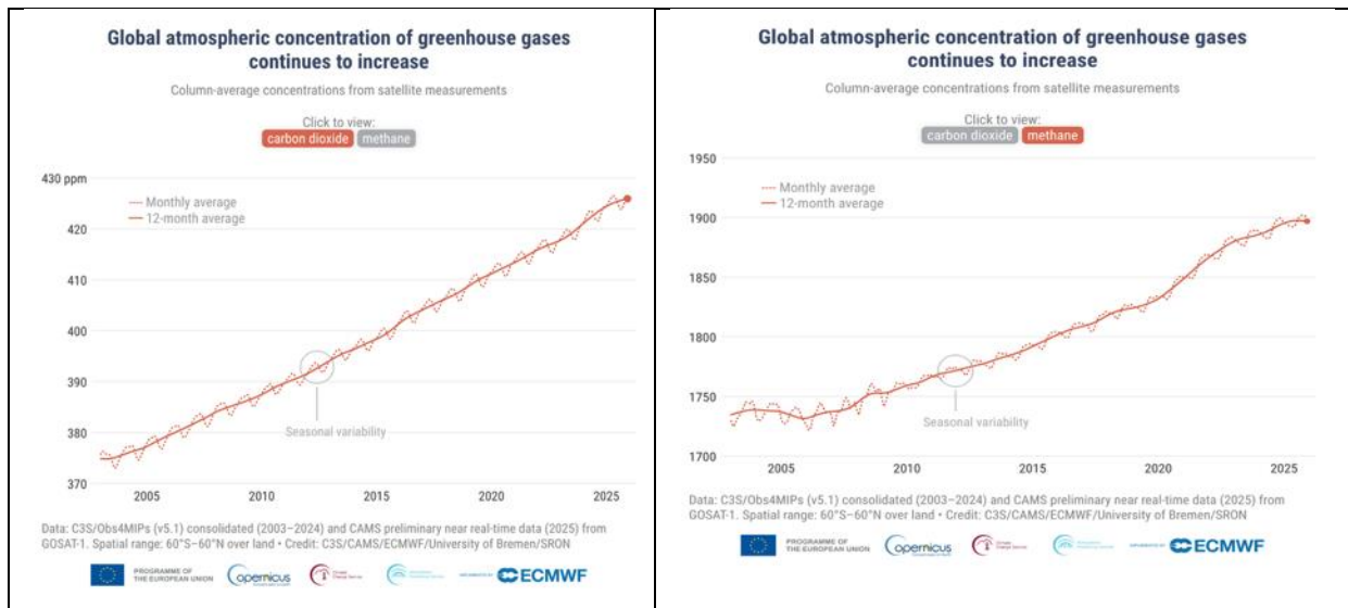
Figure 18.1. Global concentration of atmospheric column-averaged carbon dioxide (ppm) and methane (ppb) as measured by satellites for 2003–2025, with (dotted line) or without the seasonal cycle (solid line). Data: C3S/Obs4MIPs (v5.1) consolidated (2003–2024), CAMS preliminary near real-time data (2025) from GOSAT-1. Spatial range: 60°S–60°N over land. Credit: CAMS/C3S/ECMWF/University of Bremen/SRON.
