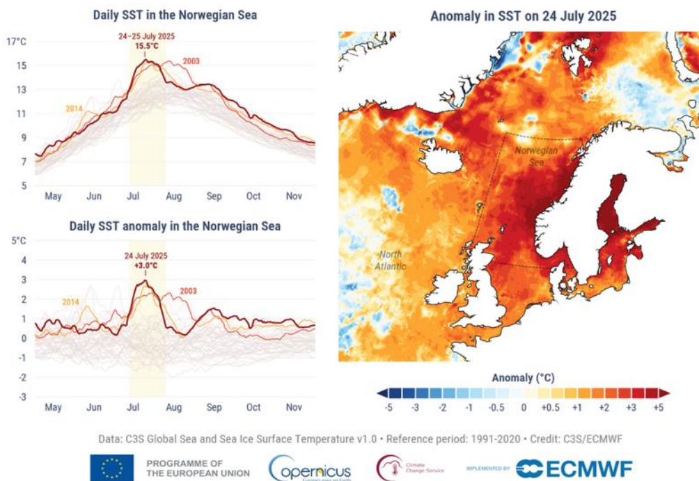
Figure 17.3. (Left) Daily sea surface temperatures ( ^{\circ}\text{C} , top) and corresponding daily anomalies ( ^{\circ}\text{C} , bottom) averaged over the Norwegian Sea for 2003 (orange), 2014 (yellow), 2025 (dark red), and all previous years since 1982 (grey). (Right) Daily sea surface temperature anomalies ( ^{\circ}\text{C} ) on 24 July 2025, the day of the highest SST across the Norwegian Sea. All anomalies are relative to the average for the 1991–2020 reference period. Data: C3S Global Sea and Sea Ice Surface Temperature v1.0. Credit: DMI/C3S/ECMWF.
