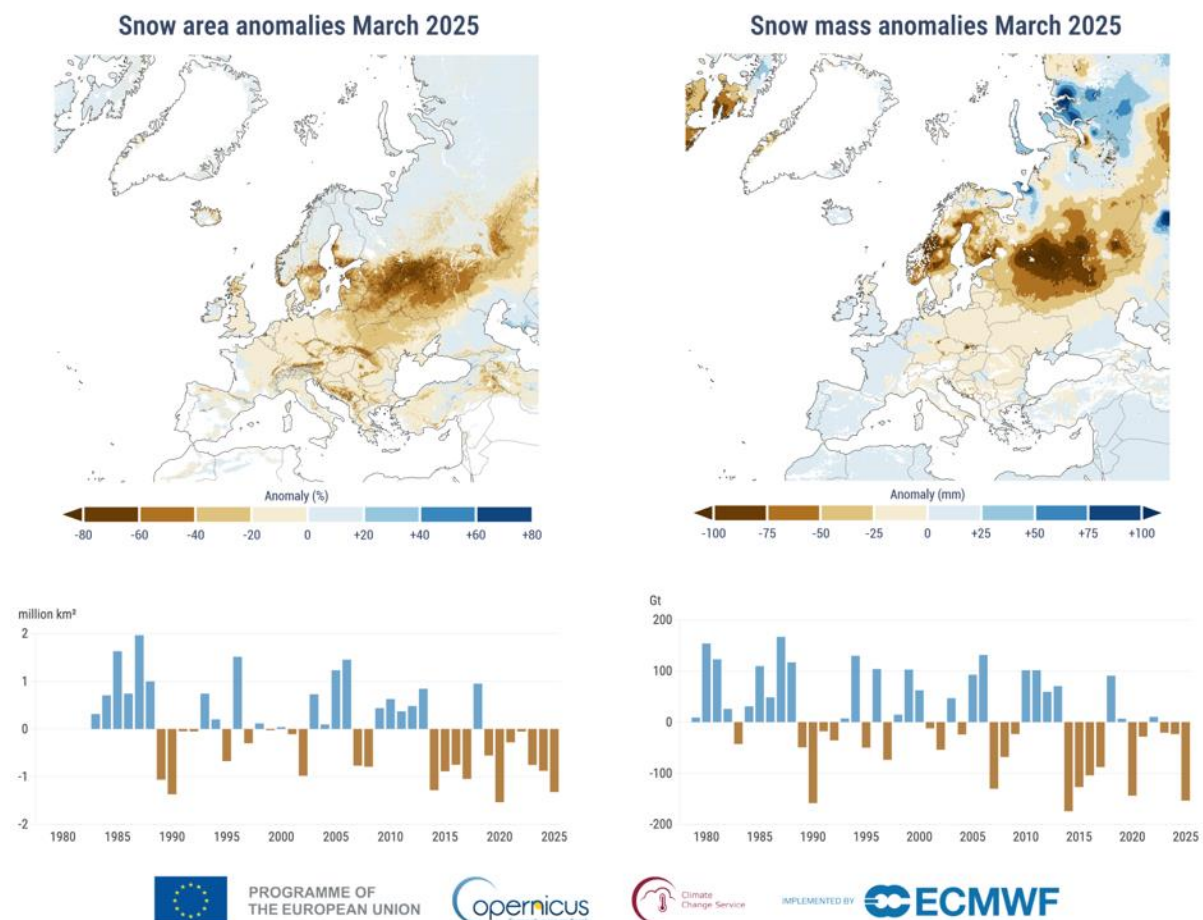
Figure 13.2. (Left) March anomalies in snow area (%) and (Right) snow mass (Gt) in 2025, relative to the average for the 1991–2020 reference period. Water bodies, glaciers and ice
