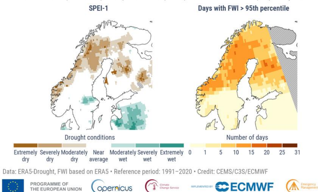
Figure 3.4. Drought conditions based on (left) the Standardised Precipitation-Evapotranspiration Index (SPEI-1) in July 2025 and (right) number of days during which the Fire Weather Index (FWI) was above the 95th percentile in July 2025. Data: ERA5-Drought, FWI based on ERA5. Credit: CEMS/C3S/ECMWF.
