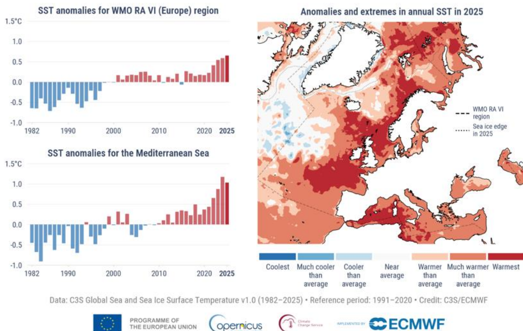
Figure 17.1. (Left) Annual average sea surface temperature (SST) anomalies ( ^{\circ}\text{C} ) for 1982–2025, relative to the average for the 1991–2020 reference period, for (top) the WMO RA VI (Europe) region and (bottom) the whole Mediterranean Sea. (Right) Anomalies and extremes in annual SST in 2025. The extreme categories (‘coolest’ and ‘warmest’) are based on rankings for 1982–2025. The other categories describe how the temperatures compare to their distribution during the 1991–2020 reference period. ‘Much cooler/warmer than average’ – cooler/warmer than 90% of temperatures; ‘cooler/warmer than average’ – than 66% of temperatures; ‘near average’ – within the middle 33%. Data: C3S Global Sea and Sea Ice Surface Temperature v1.0. Credit: DMI/C3S/ECMWF.
