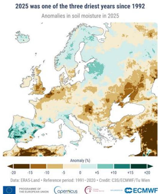
Figure 10.1a. Annual surface soil moisture anomalies (%) in 2025, showing positive (green) and negative (brown) anomalies, expressed as a percentage of the annual average for the 1991–2020 reference period. Surface soil moisture in ERA5-Land represents conditions in the upper 0–7cm of the soil. Data: ERA5-Land. Credit: C3S/ECMWF/TU Wien
