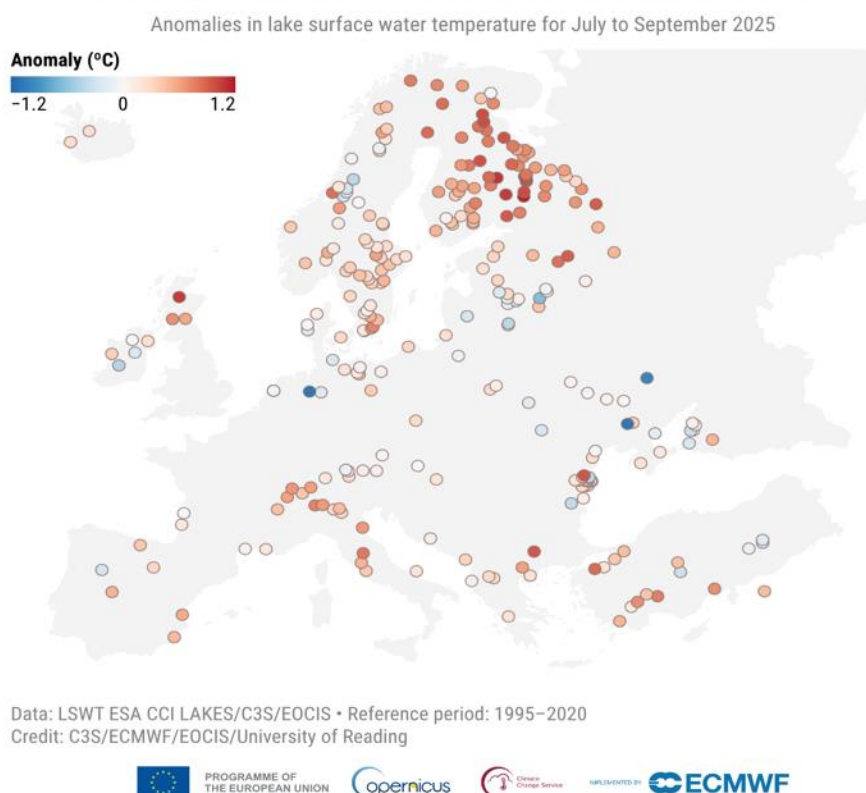
Figure 12.1. Warm season (July–September) LSWT anomalies, relative to the average for the 1995–2020 reference period, for 265 lakes in Europe. Data: ESA CCI LAKES, C3S, EOCIS lake surface water temperature data record. Credit: C3S/ECMWF/EOCIS/University of Reading.
