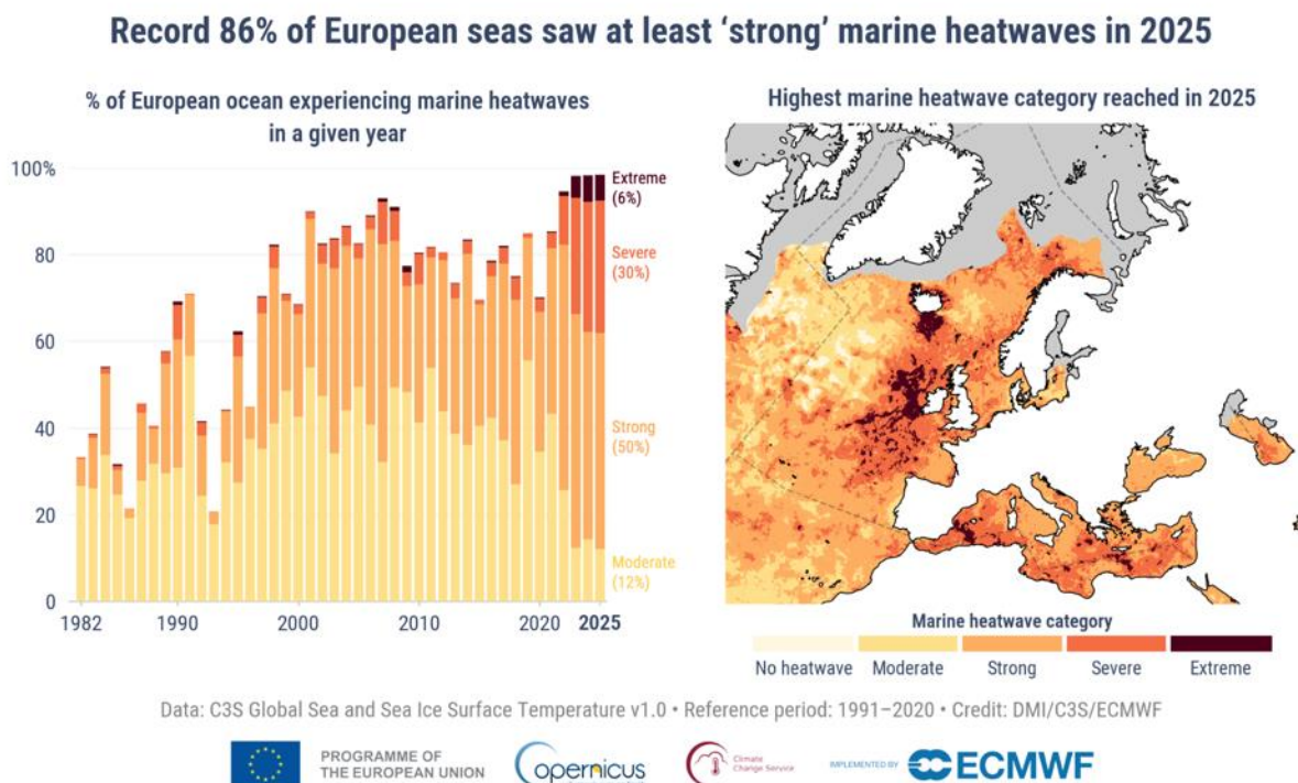
Figure 17.2. (Left) Percentage of the area of the WMO RA VI (Europe) ocean region experiencing marine heatwave conditions each year from 1982 to 2025, shown for four intensity categories: ‘moderate’ (yellow), ‘strong’ (light orange), ‘severe’ (dark orange) and ‘extreme’ (brown). For each year, the percentage is based on the highest intensity reached at each location within the region. (Right) Map showing the highest marine heatwave category experienced at each location during 2025. Marine heatwaves are defined relative to the 1991–2020 reference period. Data: C3S Global Sea and Sea Ice Surface Temperature v1.0. Credit: DMI/C3S/ECMWF.
