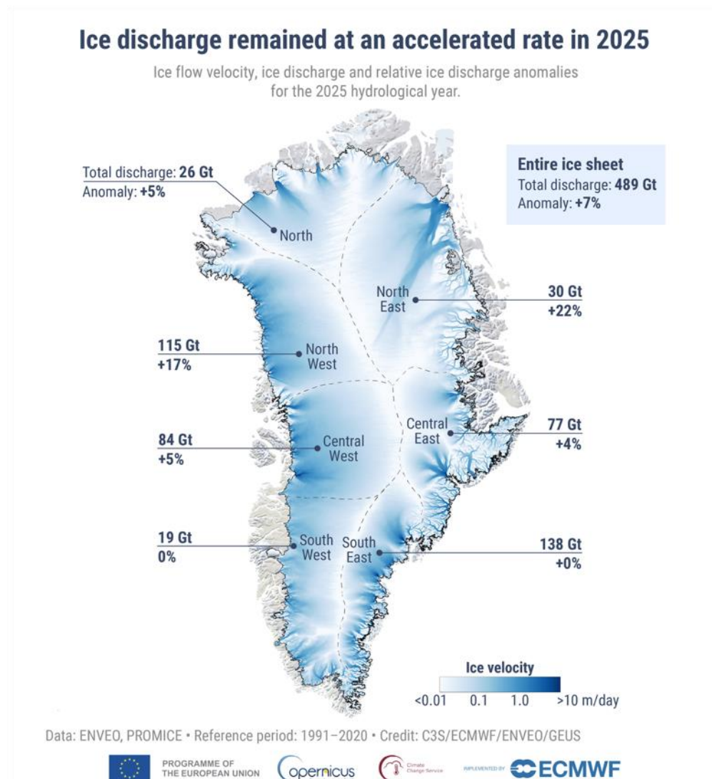
Figure 15.3. Ice flow velocity, ice discharge and relative ice discharge anomalies for the 2025 hydrological year. Ice discharge is calculated on a regional scale using drainage basins that
